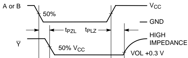
Figure 5. Switching Waveforms
